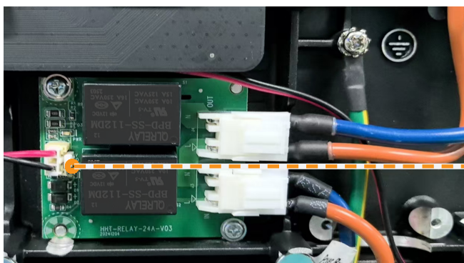
Relay wire
