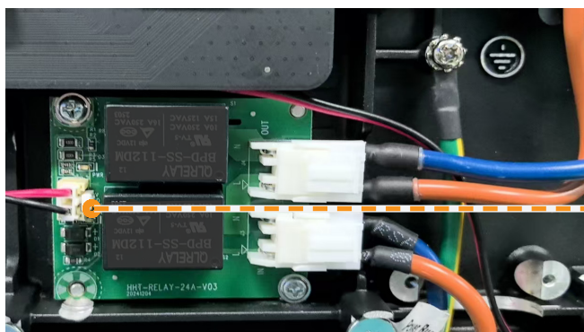
Relay wire
